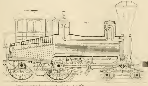
MILLHOLLAND'S ANTHRACITE PASSENGER ENGINE. FIG. 78.
